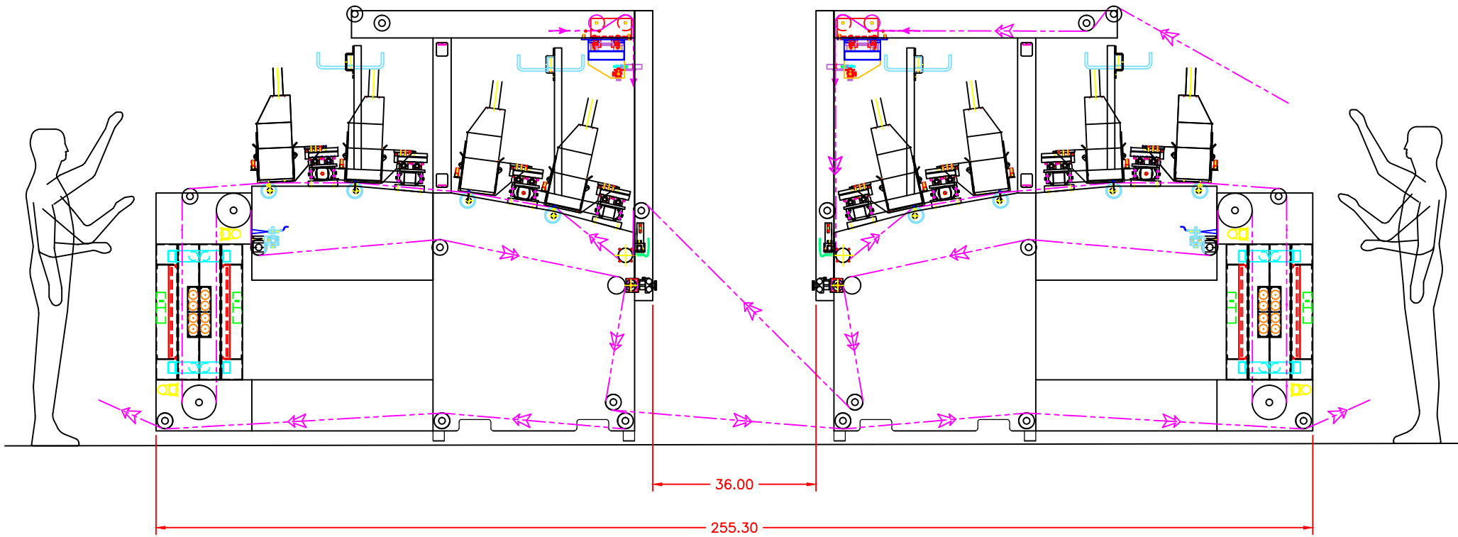
DUPLEX WITH OPTIONAL EXPANSION TO (4) RAIL (2) UNITS
