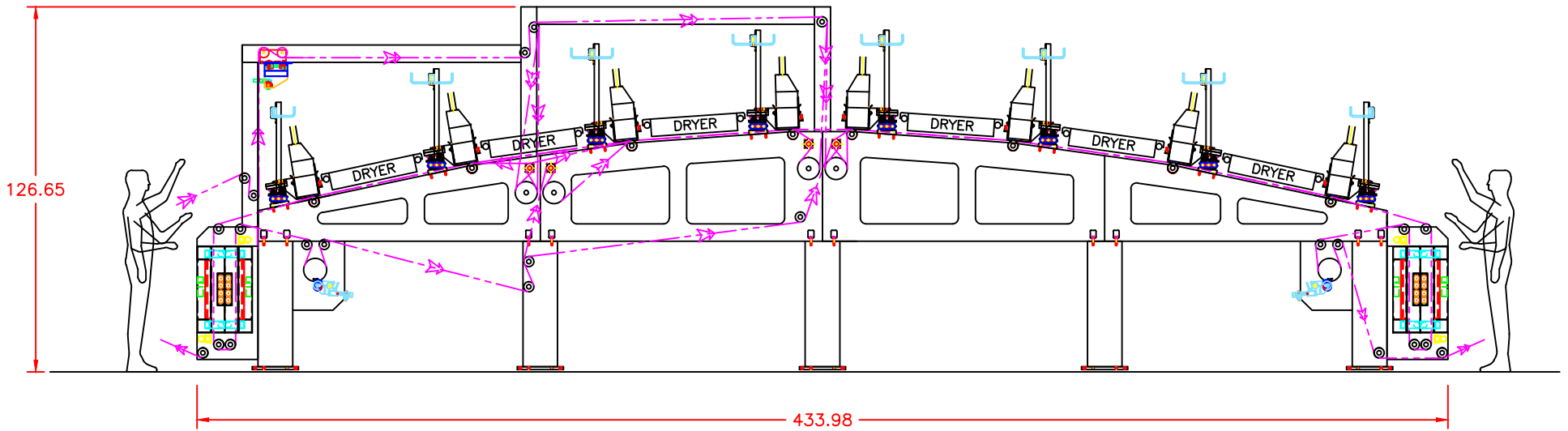
4 COLOR DUPLEX WITH INTER-DECK DRYING
